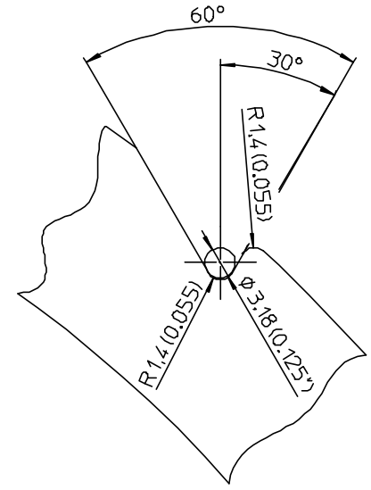
Detail A M5:1
